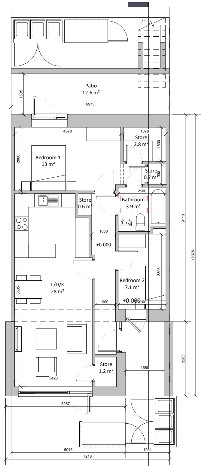
1 Ground Floor Plan (Simplex 2A) 1 : 100
